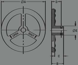
TYPE: CR6 & CR9 CAST IRON
